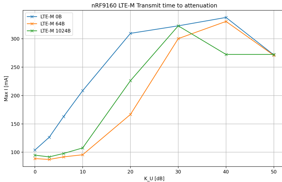
Fig. B.48: nRF9160 LTE-M Transmit time to attenuation
